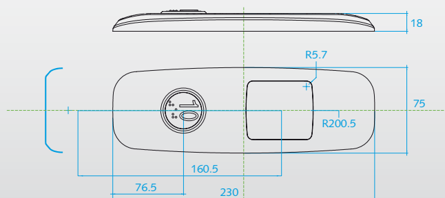
BUG#01VDI1W_L BUG#01VDI1W_S Con scasso display Icaro + scasso 1 pulsante in acciaio lucido (L), in scotch brite (S) / With hole for Icaro LCD and 1 button in mirror (L), in scotch brite (S).
